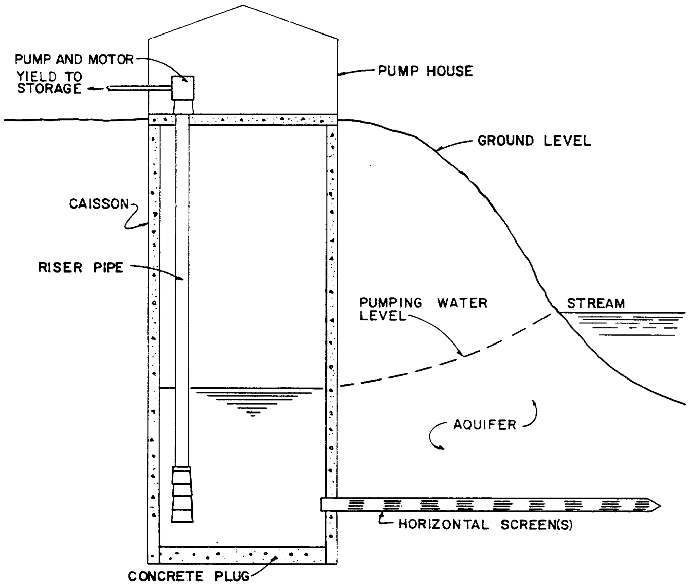
Figure 5-2. Driven well.
