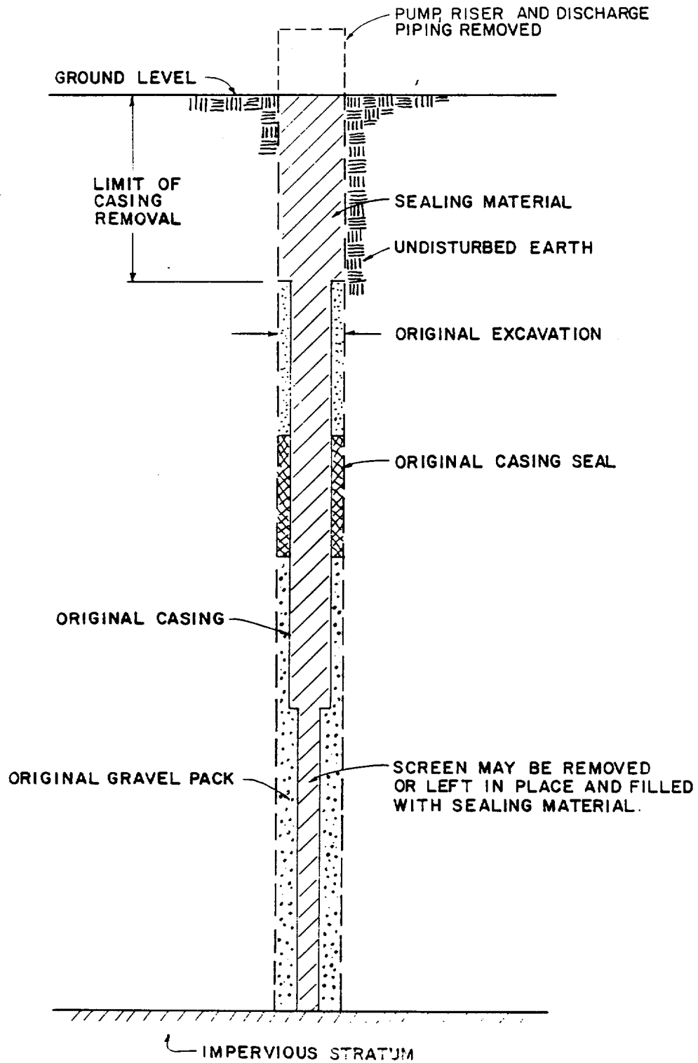
Figure 5-8. Sealed well.
